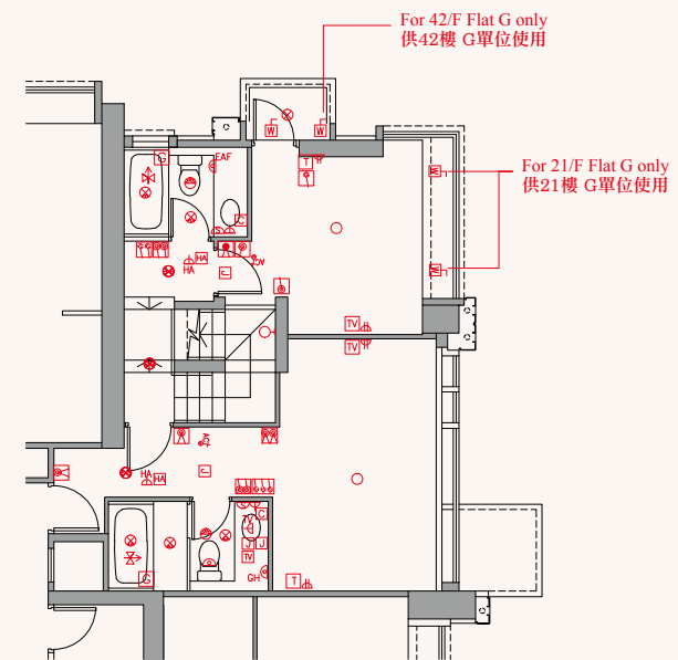
UPPER PART OF DUPLEX UNIT
