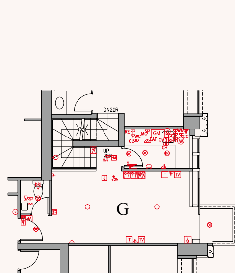
LOWER PART OF DUPLEX UNIT
