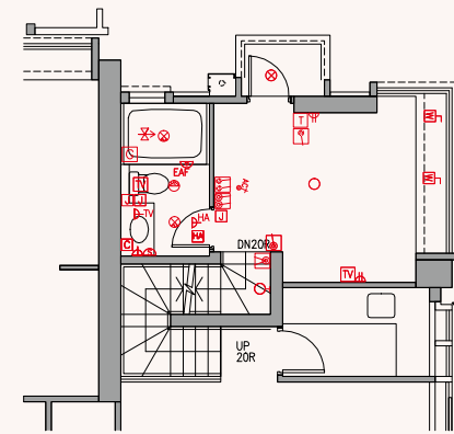
UPPER PART OF DUPLEX UNIT
