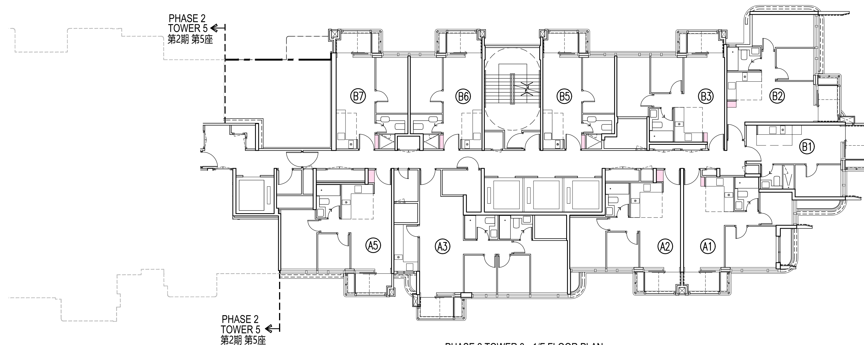
PHASE 2 TOWER 3 - 1/F FLOOR PLAN
